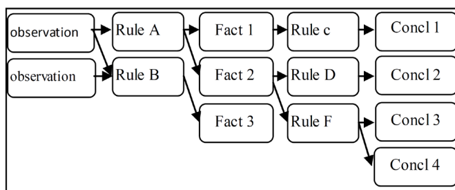
Gambar 1. Forward Chaining
