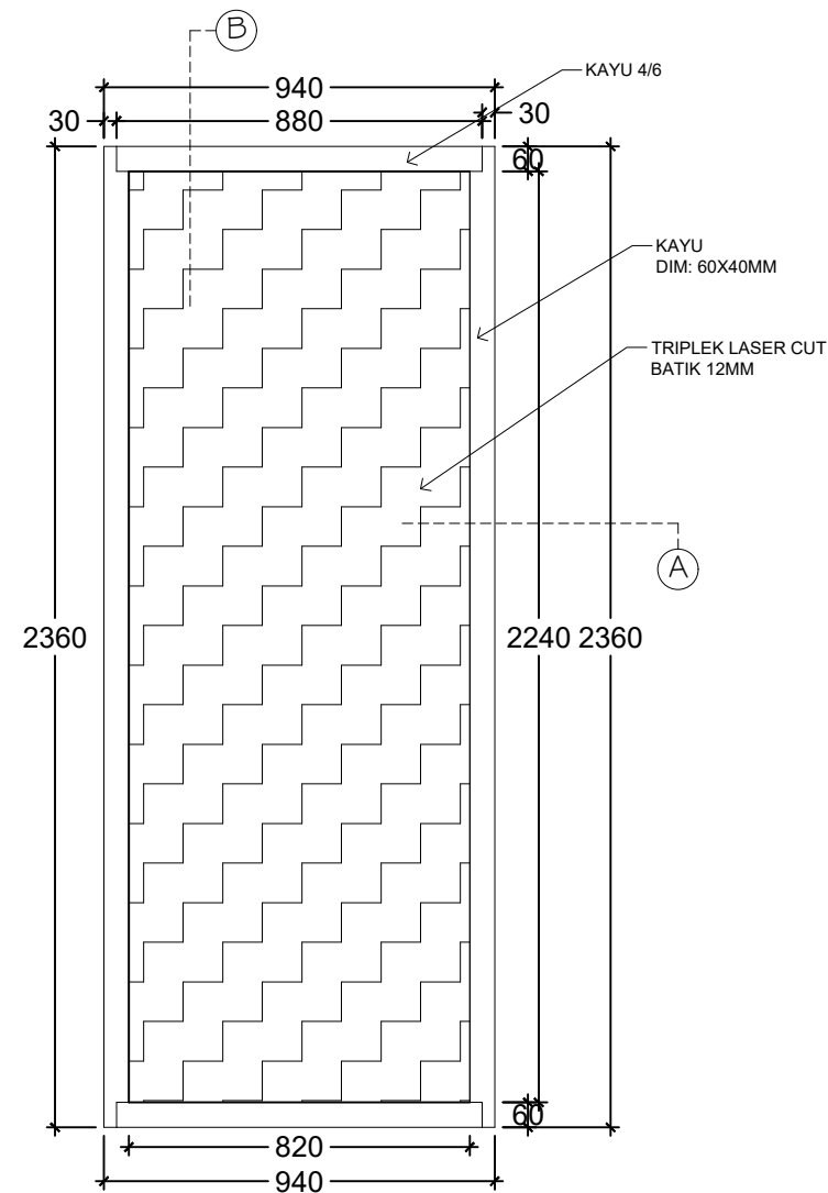
TAMPAK DEPAN BATIK SECONDARY SKIN SCALE 1: 20
