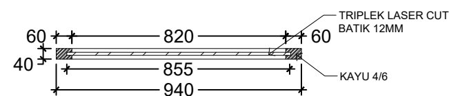
POTONGAN A SCALE 1: 20
