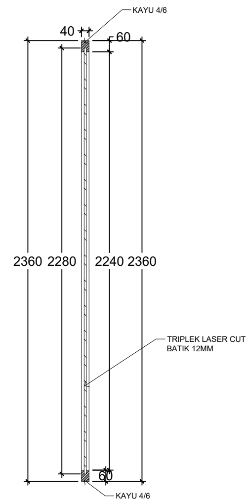
POTONGAN B SCALE 1: 20
